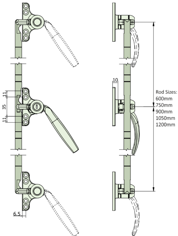
Dimensions Outward Opening 4 hole Backplate
